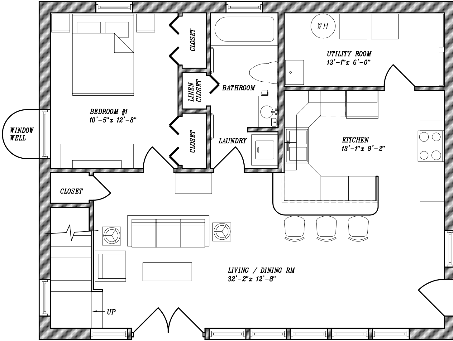
MAIN FLOOR NO SCALE
